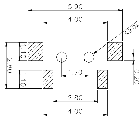
PCB. 焊接图 PCB. WELDING DRAWING
